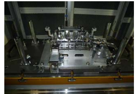
VIBRATION WELDING MACHINE
